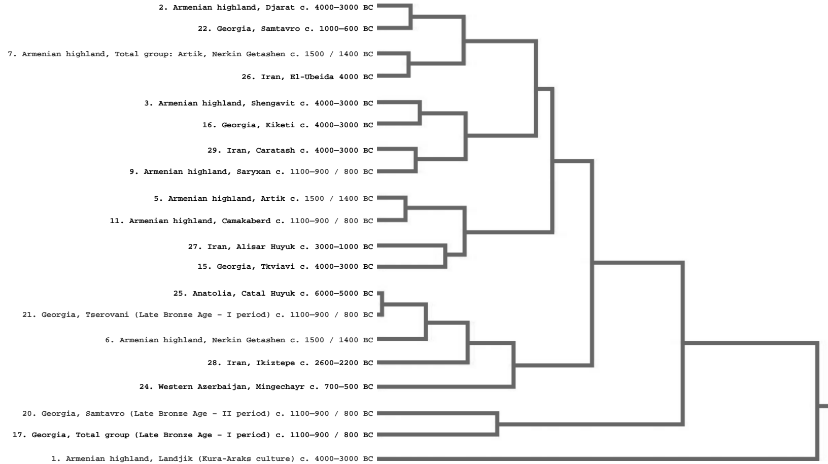
Figure 5. Analysis 2. Cophenetic correlation 0,814
