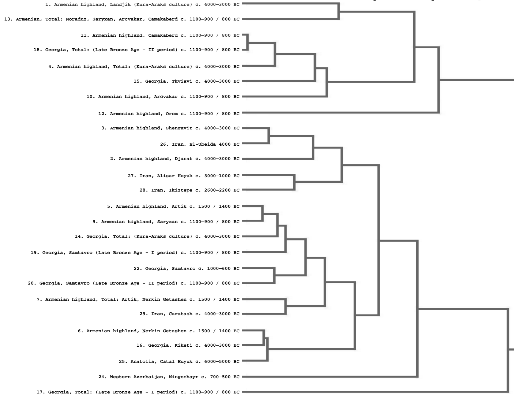
Figure 6. Analysis 3. Cophenetic correlation 0,632
