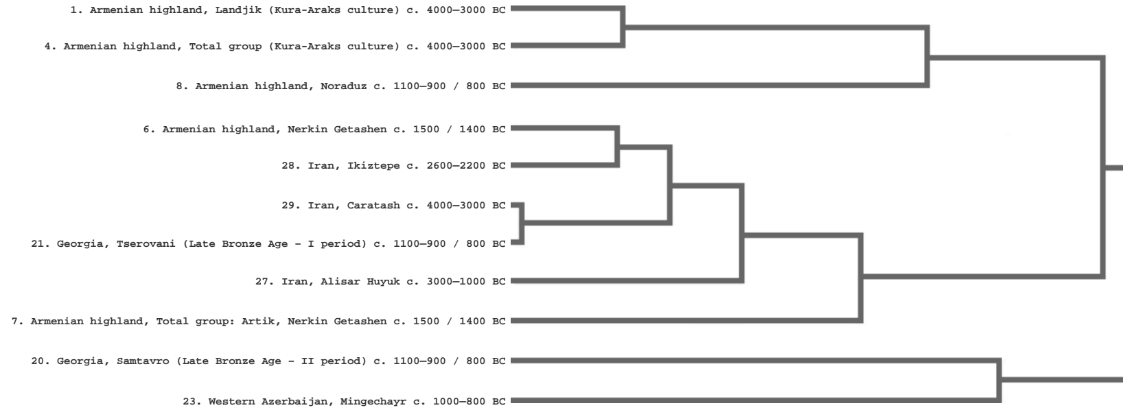
Figure 4. Analysis 1. Cophenetic correlation 0,877
